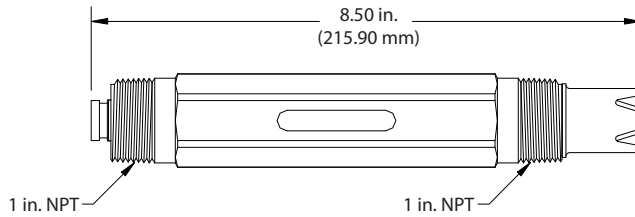
Convertible Sensor with Connector
