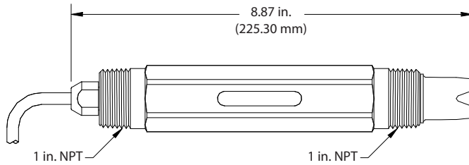
Convertible Sensor
