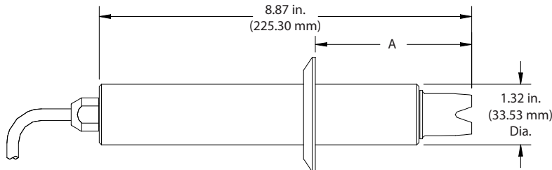
Sanitary Sensor
