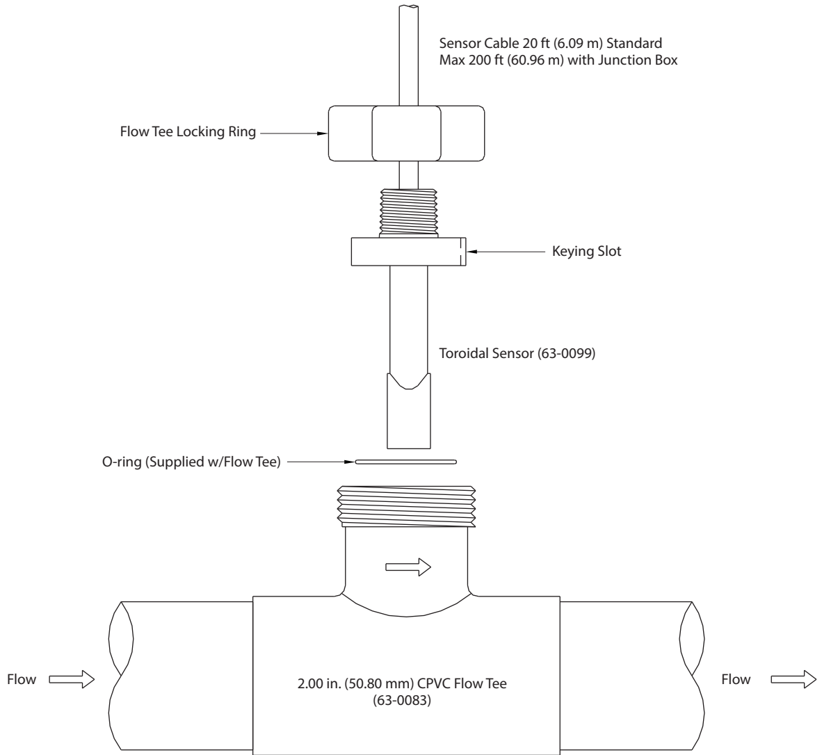
Figure 10: In-line process piping
