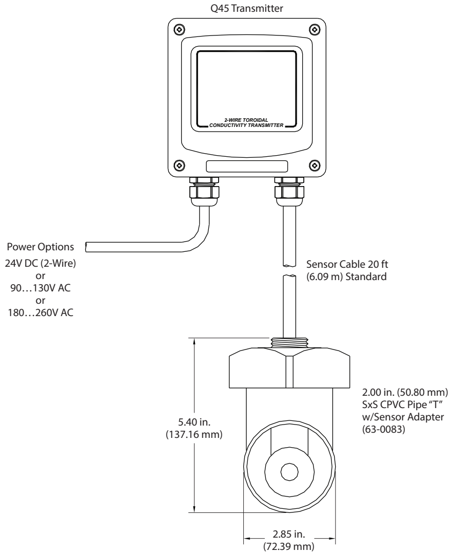
Figure 7: Sensor and flow tee assembly
