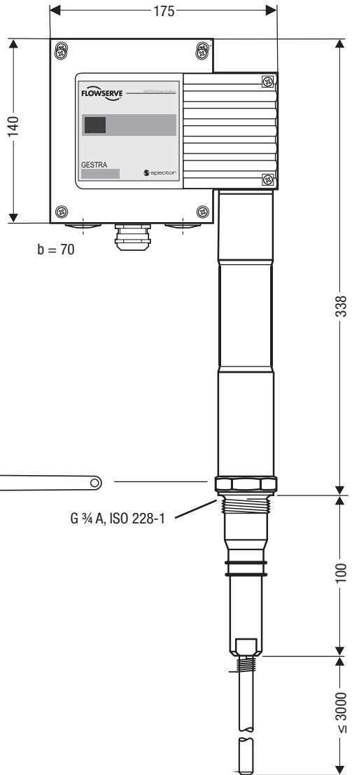
Fig. 5 NRG 16-50F, NRG 17-50F, NRG 19-50F with aluminium terminal box
