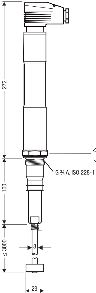
Fig. 4 NRG 16-50, NRG 17-50, NRG 19-50 with four-pole connector and measuring surface extension
